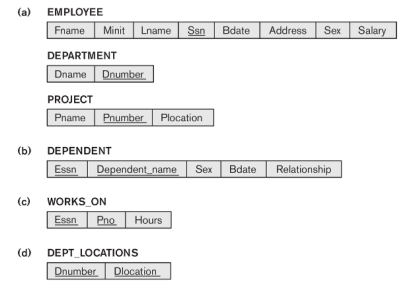
Figure 9.3 Illustration of some mapping steps. a. Entity relations after step 1. b. Additional weak entity relation after step 2. c. Relationship relation after step 5. d. Relation representing multivalued attribute after step 6.
