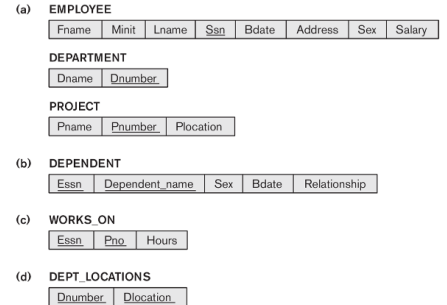
Figure 9.3 Illustration of some mapping steps. a. Entity relations after step 1. b. Additional weak entity relation after step 2. c. Relationship relation after step 5. d. Relation representing multivalued attribute after step 6.
