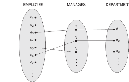
Figure 7.12 A 1:1 relationship, MANAGES.
